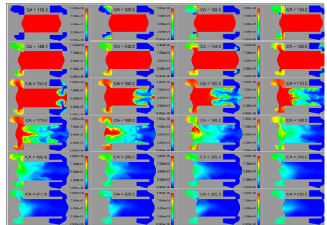
Figure 1: Full Load CFD Simulation Results of In-cylinder Gas Exchange
