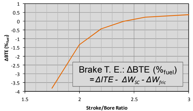
Figure 6: Combined Impact of Stroke/Bore Ratio on BTE
