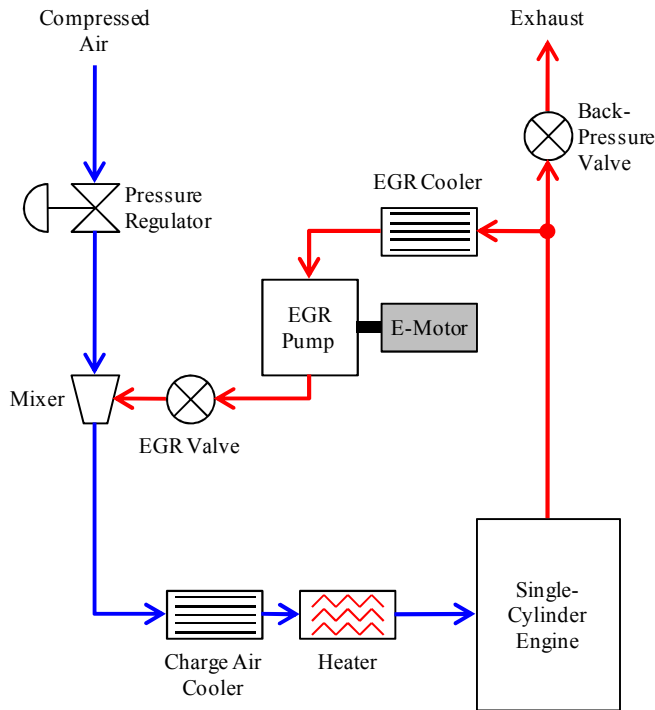
Figure 10: Schematic of the Air and EGR Conditioning System
