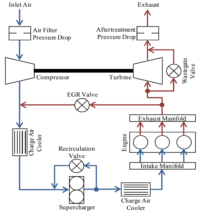
Figure 8: Air Handling System Layout
