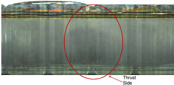
Figure 16: Intake Piston Unrolled (Color Enhanced) – Post Test
