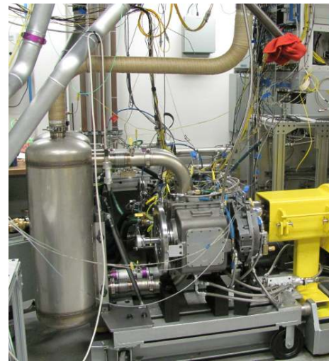
Figure 9: Single-Cylinder Research Engine Installed in Test Cell
