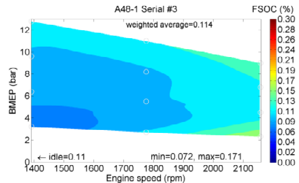
Figure 15: Fuel-specific Oil Consumption Map of the A48 1.6L SCE Engine
