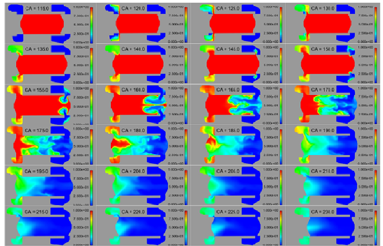
Figure 1 -Full Load CFD Simulation Results of In-cylinder Gas Exchange
