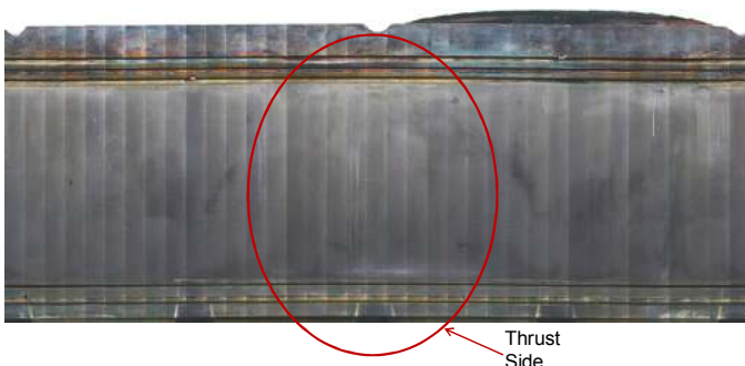
Figure 17: Exhaust Piston Unrolled (Color Enhanced) – Post Test
