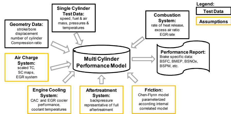
Figure 11: Multi-cylinder Interface Model Input Data Flow
